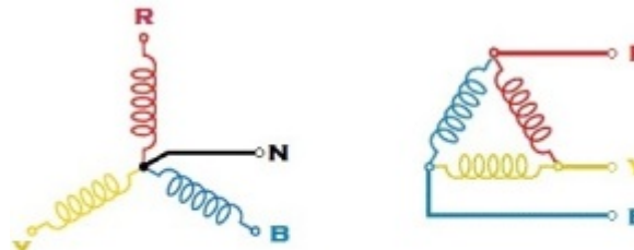
Comparison b/w Star (Y) & Delta (Δ) Connections © www.electricaltechnology.org
