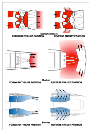
Figure 22.1 The Three Types of Reverse Thrust Systems
